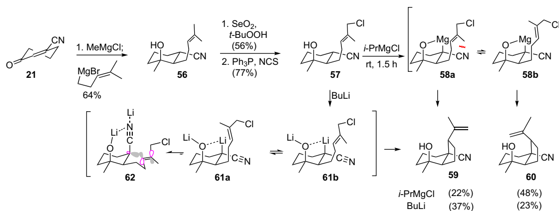
Scheme 14. Metalated nitrile cyclizations to cis -hydrindanes.
