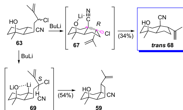
Scheme 16. Nitrile cyclizations to cis - and trans -hydrindanes.
