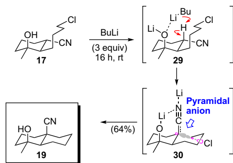
Scheme 7. trans -Selective cyclization with a dilithiated nitrile anion.
