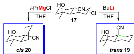
Scheme 4. Cation-controlled cyclizations.
