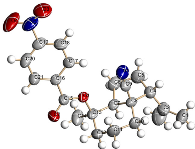
Figure 2. ORTEP of the trans -hydrindane 66 .
