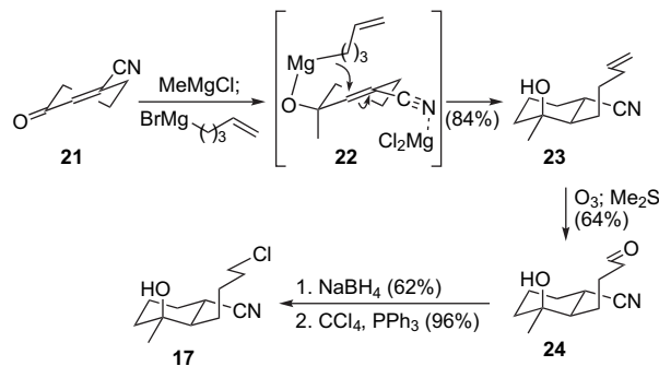
Scheme 5. Synthesis of nitrile cyclization prototype 17 .
