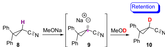
Scheme 2. Retentive deuteration of a nitrile anion.
