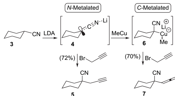
Scheme 1. Regiodivergent alkylations of N - and C-metalated nitriles.
