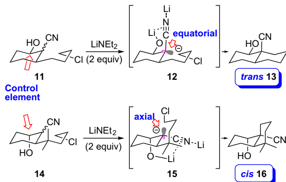
Scheme 3. Chelation-controlled cyclizations of nitrile anions.
