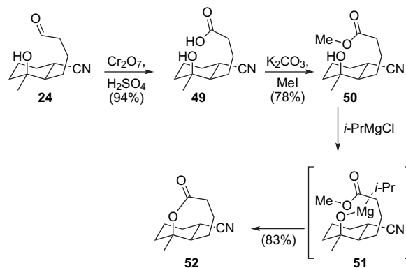
Scheme 12. Intramolecular lactonization with an ester nitrile.
