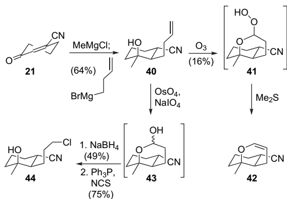
Scheme 10. Synthesis of the hydrindane cyclization precursor 44 .
