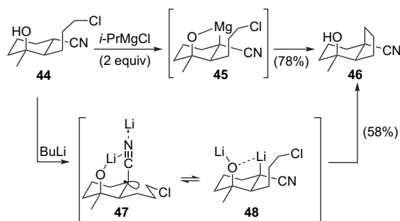
Scheme 11. Cyclizations to cis -hydrindane 46 .
