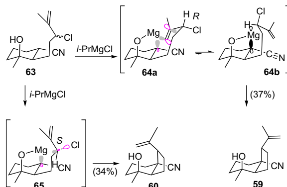
Scheme 15. Cyclizations of allylic chlorides to cis -hydrindanes.
