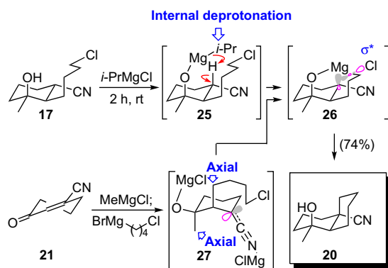
Scheme 6. cis -Selective cyclizations of magnesiased nitriles.
