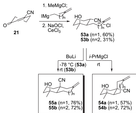
Scheme 13. Stereodivergent decalin and bicyclo[5.4.0]undecane syntheses.
