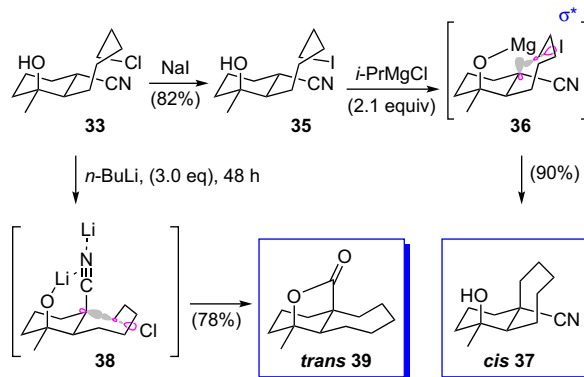
Scheme 9. Stereodivergent cyclizations to bicyclo[5.4.0]undecanes.
