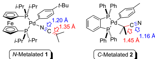
Figure 1. Structures of metalated nitriles.
